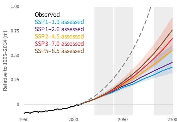
d) Global mean sea level change
